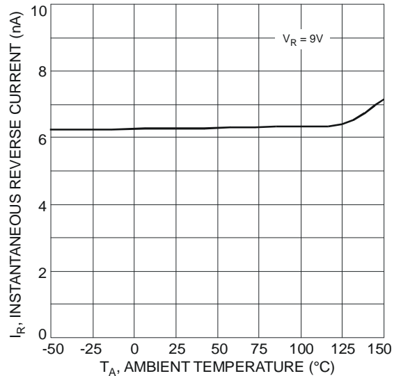
Fig. 4 Instantaneous Reverse Current vs. Ambient Temperature
